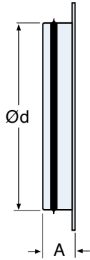
Connection spigot BRAS
